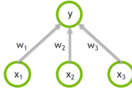
Artificial neuron
