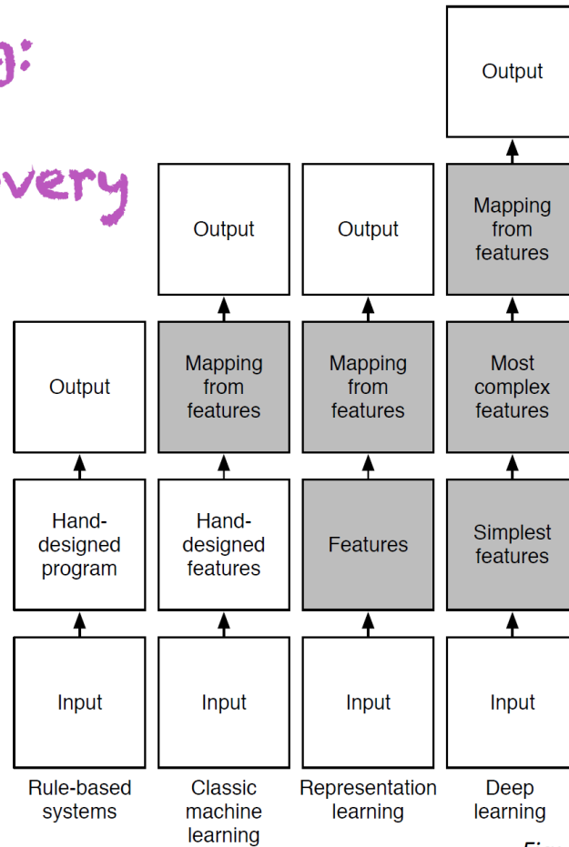
Fig. 1. Goodfellow
